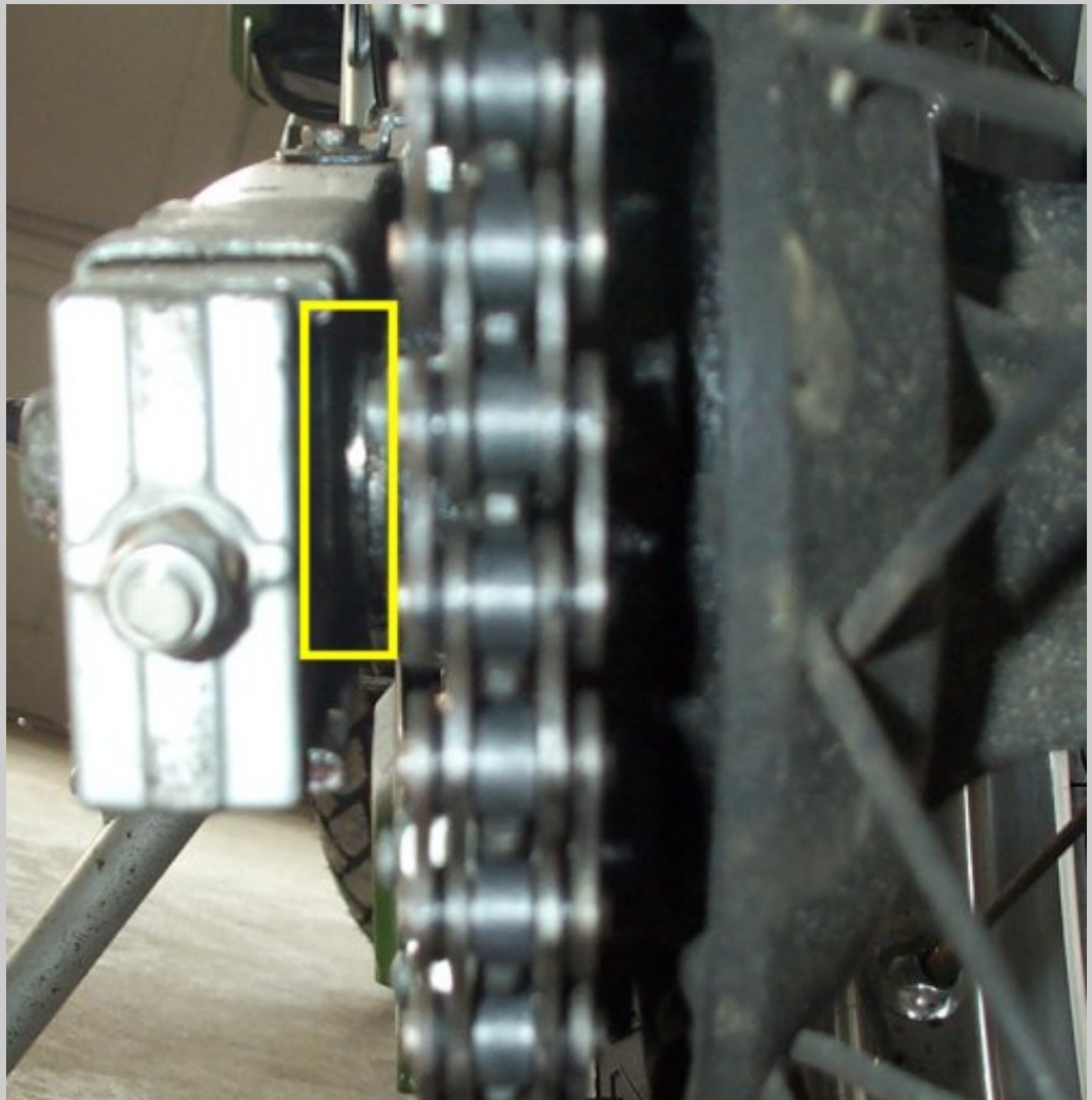
The right rear wheel spacer is shown above. This must be replaced when changing tires or whatever.
