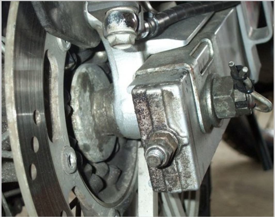
The right rear wheel spacer is shown above. This must be replaced when changing tires or whatever.
