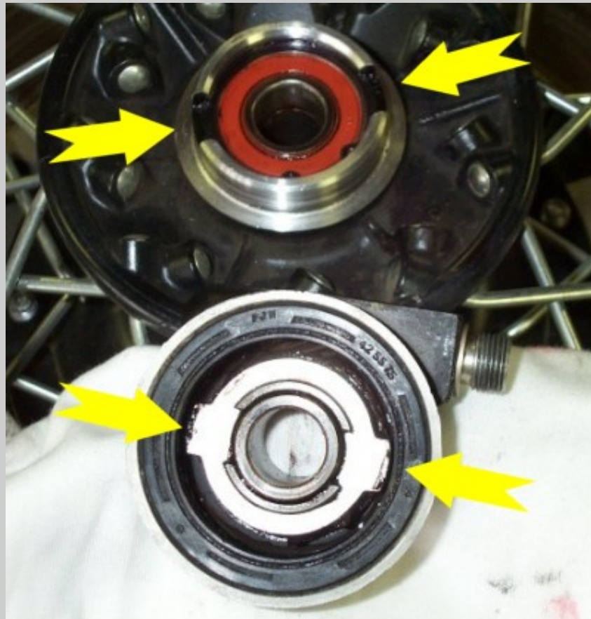
The above picture shows the inside of the speedometer hub, (located normally on the right side of the front wheel.) The yellow arrows point to the tab ears, and the slots into which they fit.
